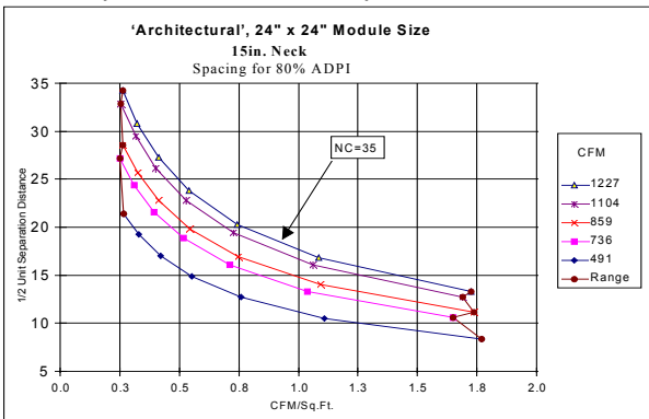
Fig 2 Architectural Diffuser
