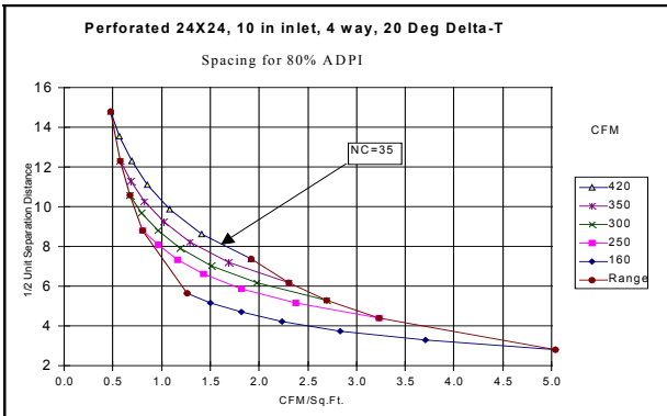
Fig 1 Perforated Diffuser
